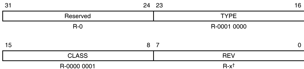
Figure B–247. PLL Controller Peripheral Identification Register (PLLPID)
