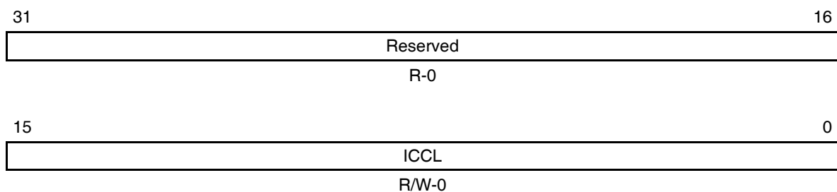
Figure B-141. I2C Clock Low-Time Divider Register (I2CCLKL)
