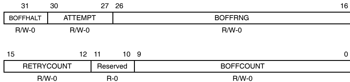
Figure B–101. Backoff Test Register (BOFFTEST)
