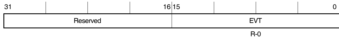
Figure B–51. EDMA Event Register (ER)
