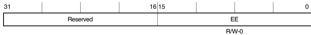
Figure B–53. EDMA Event Enable Register (EER)
