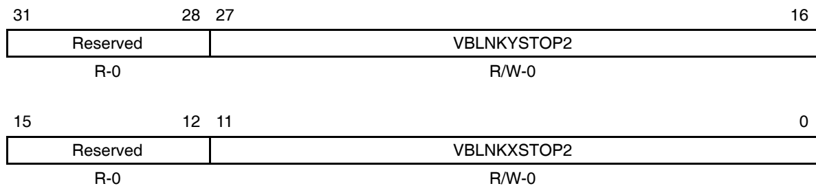
Figure B–326. Video Display Field 2 Vertical Blanking End Register (VDVBLKE2)
