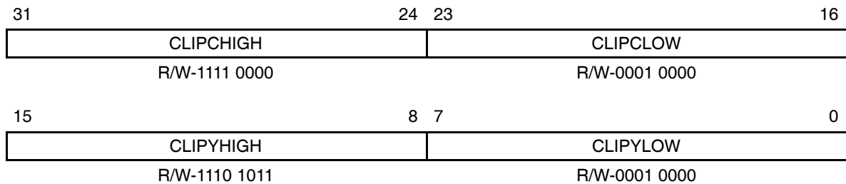
Figure B–341. Video Display Clipping Register (VDCLIP)
