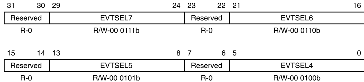
Figure B–37. EDMA Event Selector Register 1 (ESEL1)
