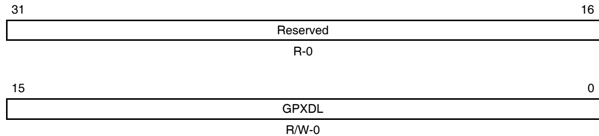
Figure B–129. GPIO Delta Low Register (GPD_L)
