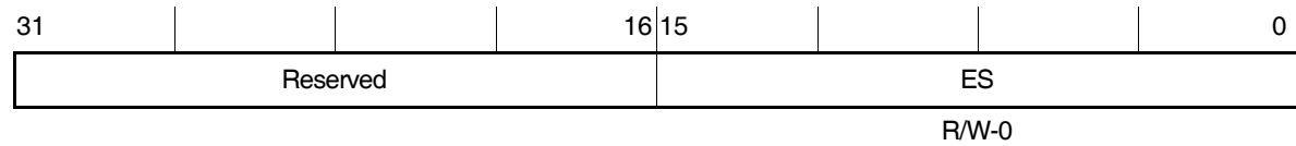
Figure B–59. EDMA Event Set Register (ESR)
