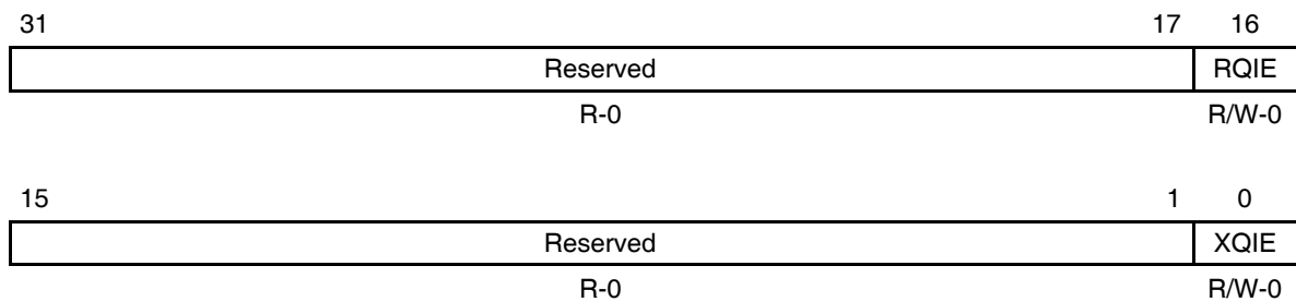
Figure B–274. UTOPIA Interrupt Enable Register (UIER)
