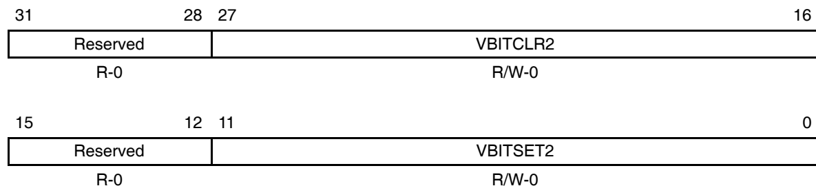
Figure B–347. Video Display Field 2 Vertical Blanking Bit Register (VDVBIT2)
