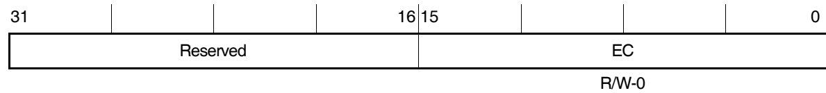
Figure B–56. EDMA Event Clear Register (ECR)
