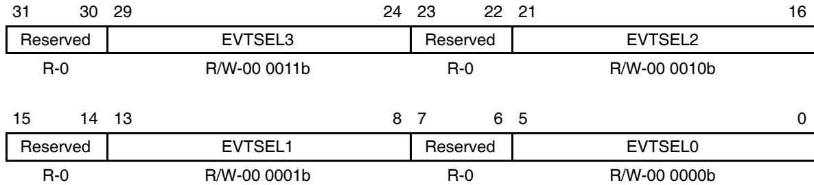
Figure B–36. EDMA Event Selector Register 0 (ESEL0)
