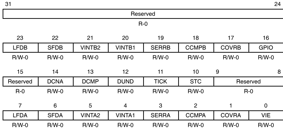
Figure B–297. Video Port Interrupt Enable Register (VPIE)
