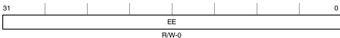
Figure B–54. EDMA Event Enable Low Register (EERL)
