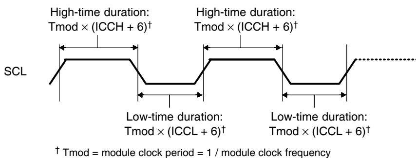
Figure B-140. Roles of the Clock Divide-Down Values (ICCL and ICCH)
