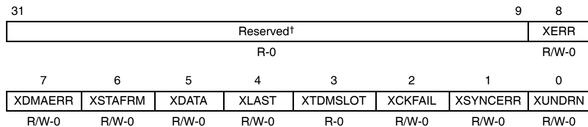
Figure B–195. Transmitter Status Register (XSTAT)
