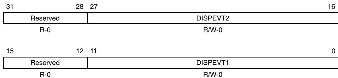
Figure B–340. Video Display Display Event Register (VDDISPEVT)
