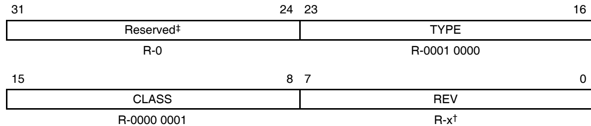
Figure B–163. Peripheral Identification Register (PID)
