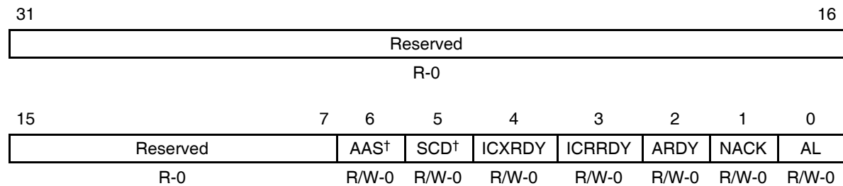
Figure B–138. I2C Interrupt Enable Register (I2CIER)
