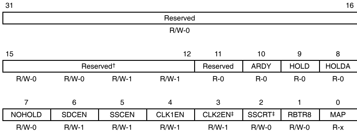
Figure B–110. EMIF Global Control Register (GBLCTL)
